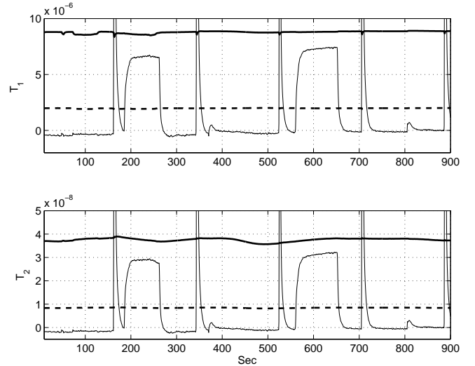
Fig. 5. Simplified test quantities (solid thin line) with adaptive alarm thresholds (solid thick line, \phi_{\min} = 0 , dashed thick line, \phi_{\min} = 0.5 )
