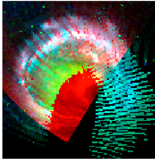
Figure 1. RGB spectrometer-imager composition of the southern aurora. The red channel comes from an imager acquisition of the aurora (4.54–5.02 \mu\text{m} ). Green is set at 3.31 \mu\text{m} where the \text{H}_3^+ emission is overlaid to the \text{CH}_4 Q branch, and blue is set at 3.54 \mu\text{m} , a \text{H}_3^+ emission band. The green and blue channels are composed from the spectrometer's data. The spectral data do not completely cover the imager acquisition. Colors would be affected by both brightness and relative amplitude of the RGB bands. Black corresponds to the absence of data.
