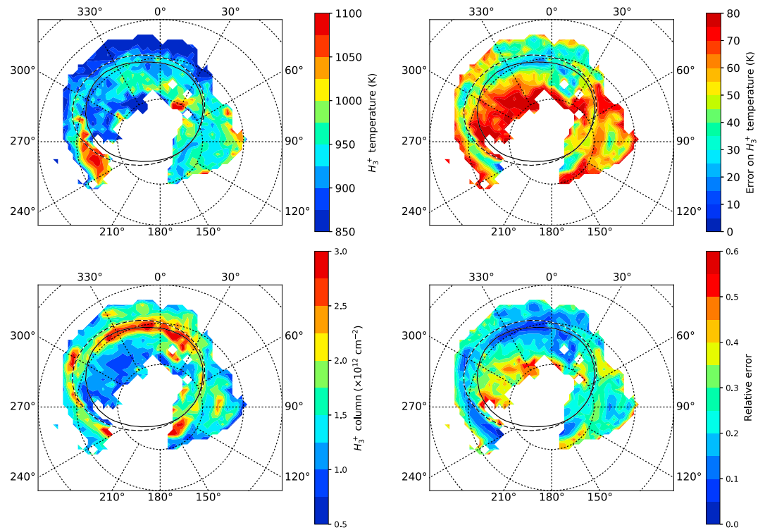
Figure 4. (top left) H_3^+ effective temperature and (top right) error on its retrieval. (bottom left) H_3^+ column density and (bottom right) error on its retrieval. The continuous oval curve is from VIP4 model [Connerney et al. , 1998]; the dashed curve is the UV statistical oval reported by Grodent et al. [2003]. Latitude lines are spaced by 10^\circ . The orthographic projection that contains the 60^\circ latitude south circle is divided into 50 \times 50 bins for each map. Then, all the measurement points falling in each single bin are averaged to produce the contour plots shown in the figure.
