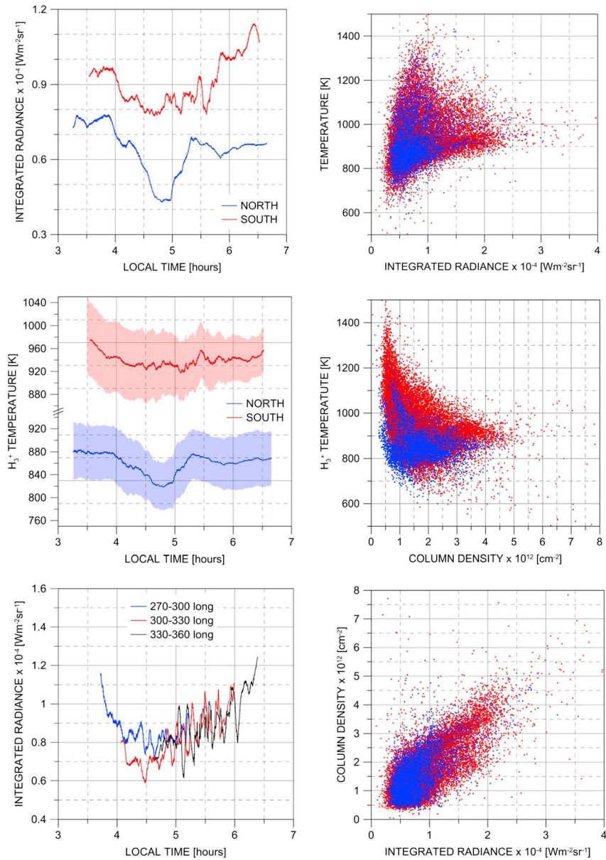
Figure 5. (left column, top) Local time dependence of the H 3 + integrated radiance (emissions in the range 3.35 and 3.75 μm) versus the Jovian time of the day; (left column, middle) H 3 + effective temperature versus the Jovian time of the day, the colored regions account for the respective retrieval errors on the temperature; (left column, bottom) trends of the integrated radiances during the Jovian day in three different longitudinal sectors of the southern aurora. The error on the integrated radiances reported in the panels is less than 0.7 \times 10^{-5} \text{ W m}^{-2} \text{ sr}^{-1} . (right column, top) Scatterplots between temperature and integrated radiance, (right column, middle) temperature and column density, and (right column, bottom) column density and integrated radiance. In the scatterplots the northern auroral data are shown in blue and southern ones are in red.
