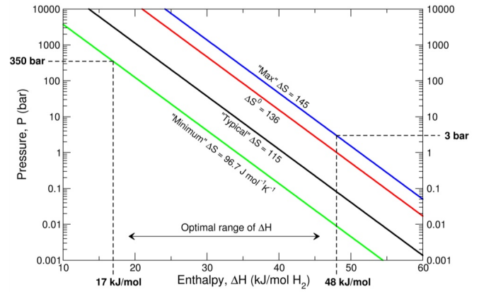
Fig. 3: Equilibrium H_2 desorption pressure ( P ) for a generic hydrogen storage material as a function of desorption enthalpy ( \Delta H ) for various choices of desorption entropy ( \Delta S ) at T = 80^\circ C . Adapted from Ref. [7]. The minimum pressure for the fuel cell inlet is taken to be 3 bar; the refueling pressure is assumed to be 350 bar.
