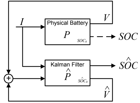
Fig. 6: Block diagram of SOC estimation scheme using the electrode average model and a Kalman filter.
