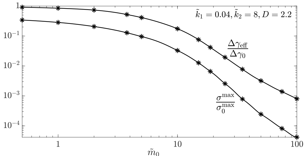
Figure 5: The effect of dimensionless height variance \tilde{m}_0 on \sigma^{\text{max}} and \Delta\gamma_{\text{eff}} for fractal roughness with D = 2.2 and \tilde{k}_1 = 0.04 , \tilde{k}_2 = 8 .
